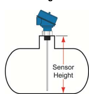
Riser Raises Sensor Height
