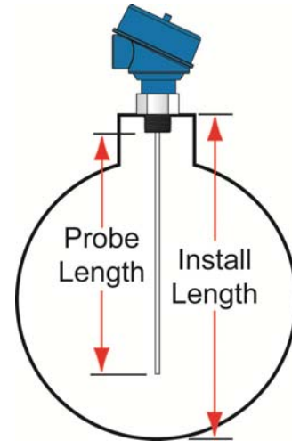
Horizontal Tank
