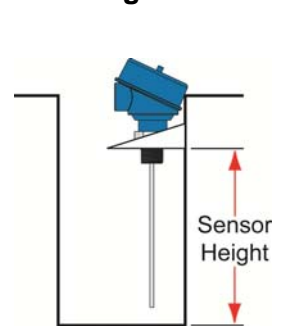
Riser Raises Sensor Height
