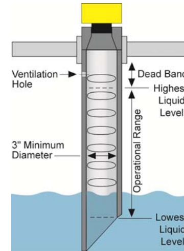
Mounting with a Standpipe
